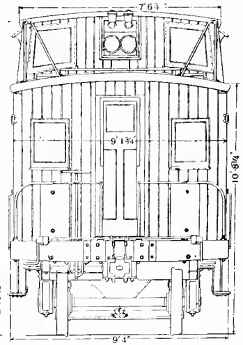
Fig. 82. End Elevation.
